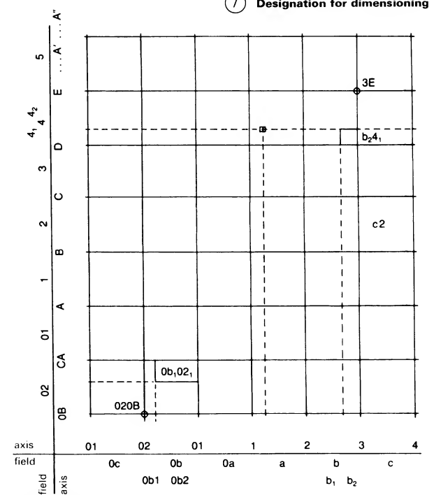
8 Axis-field grid
